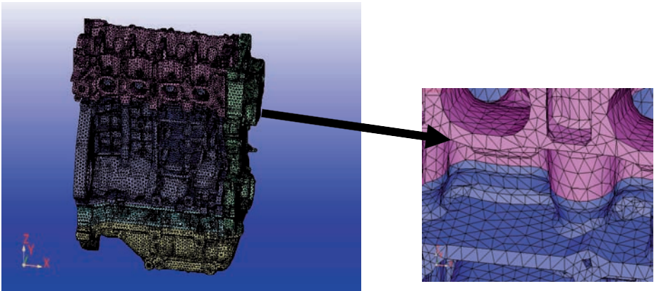
Fig. 4.5.4.1: Example of automatic assembly meshing (courtesy of Techno-Star Europe GmbH)
