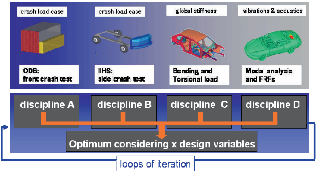
Fig. 4.2.2.2: Multi-disciplinary Optimization in Vehicle Design
