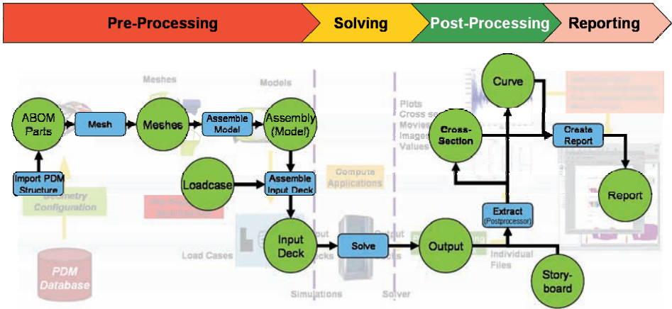
Fig. 4.5.2.1: Simulation Data and Process Management (courtesy of MSC Software)
