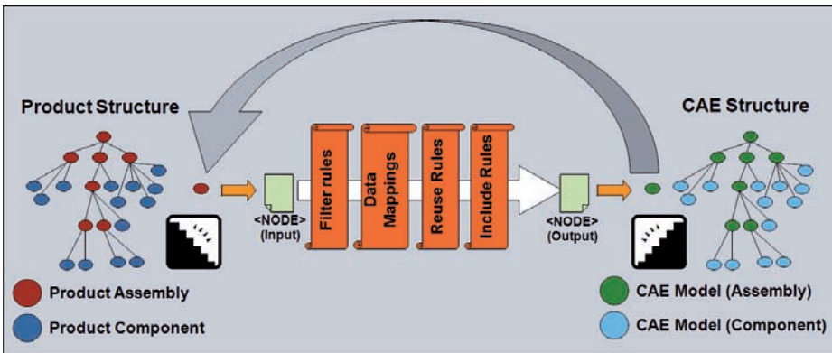
Fig.4.5.4.2 Product structure and CAE (courtesy of Siemens PLM Software)
