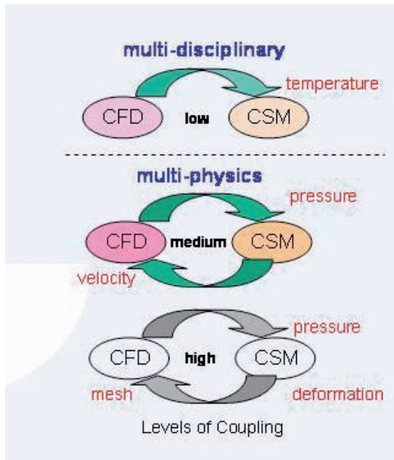
Fig.4.2.2.1: Levels of physical coupling
