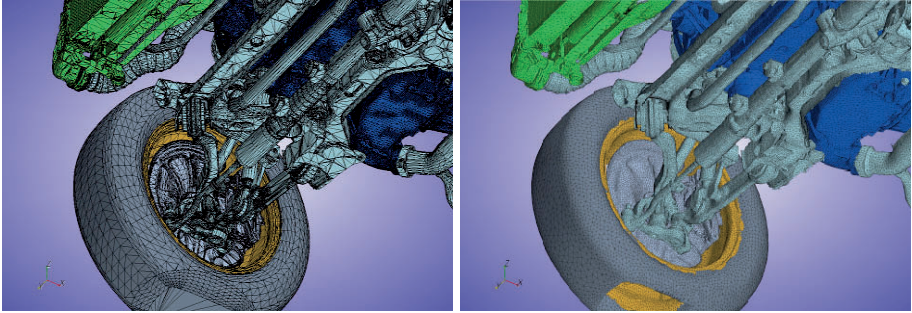
Fig.4.5.6.2 Imported CAD (left) and wrapped surface (right) with detailed feature retention and implicit small-scale de-featuring
